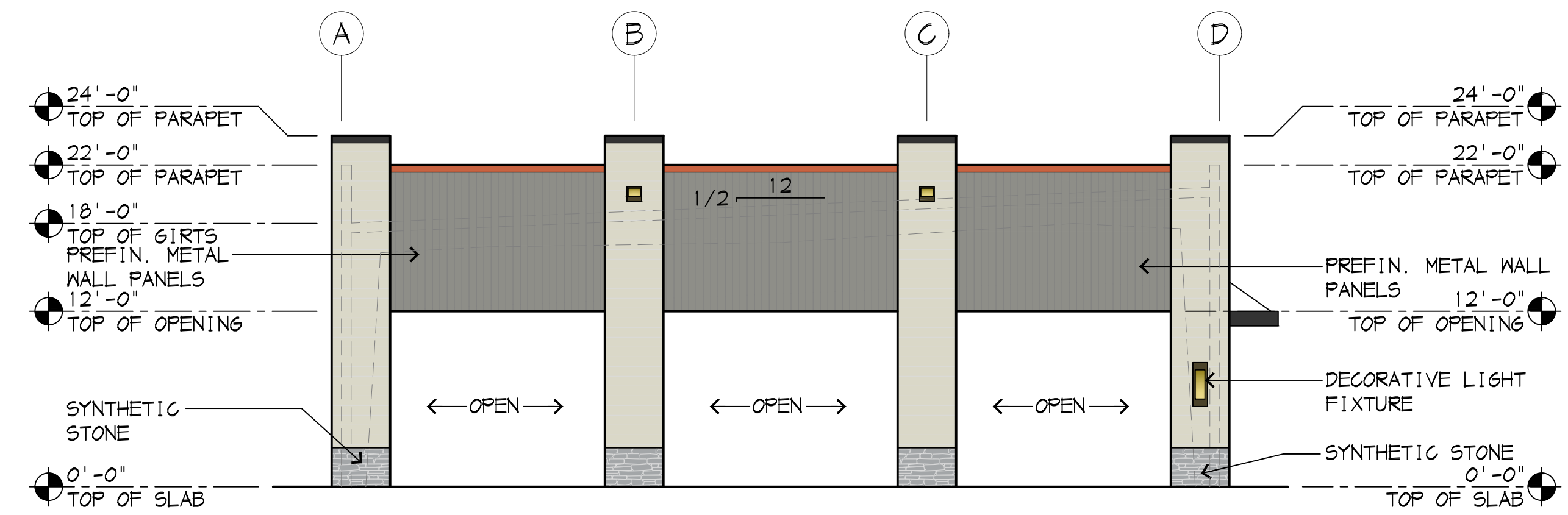
BUILDING A SOUTH ELEVATION
