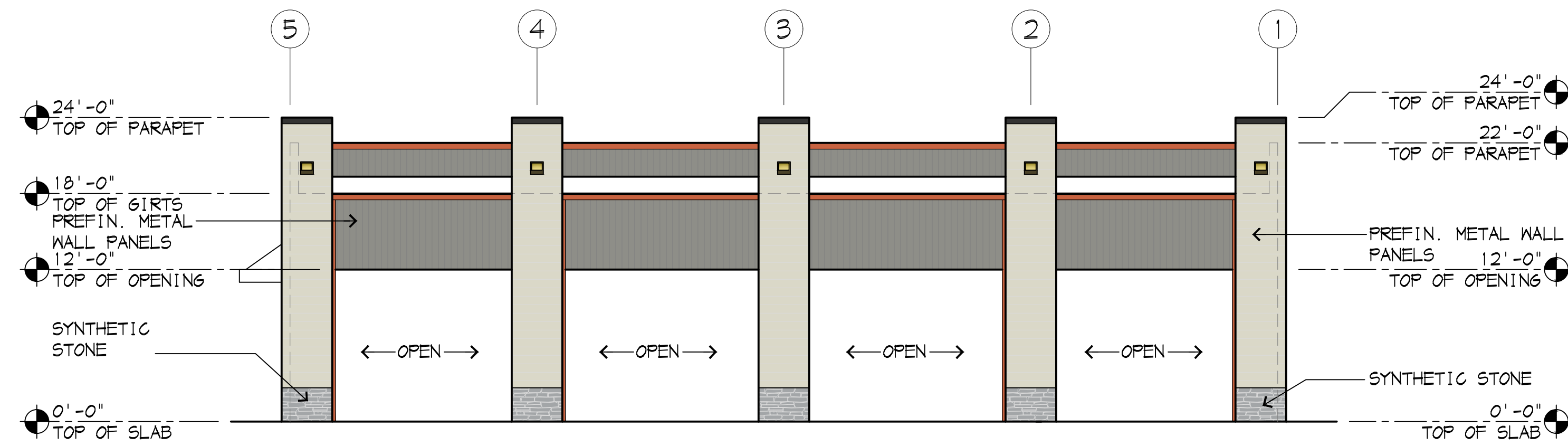
BUILDING A WEST ELEVATION
